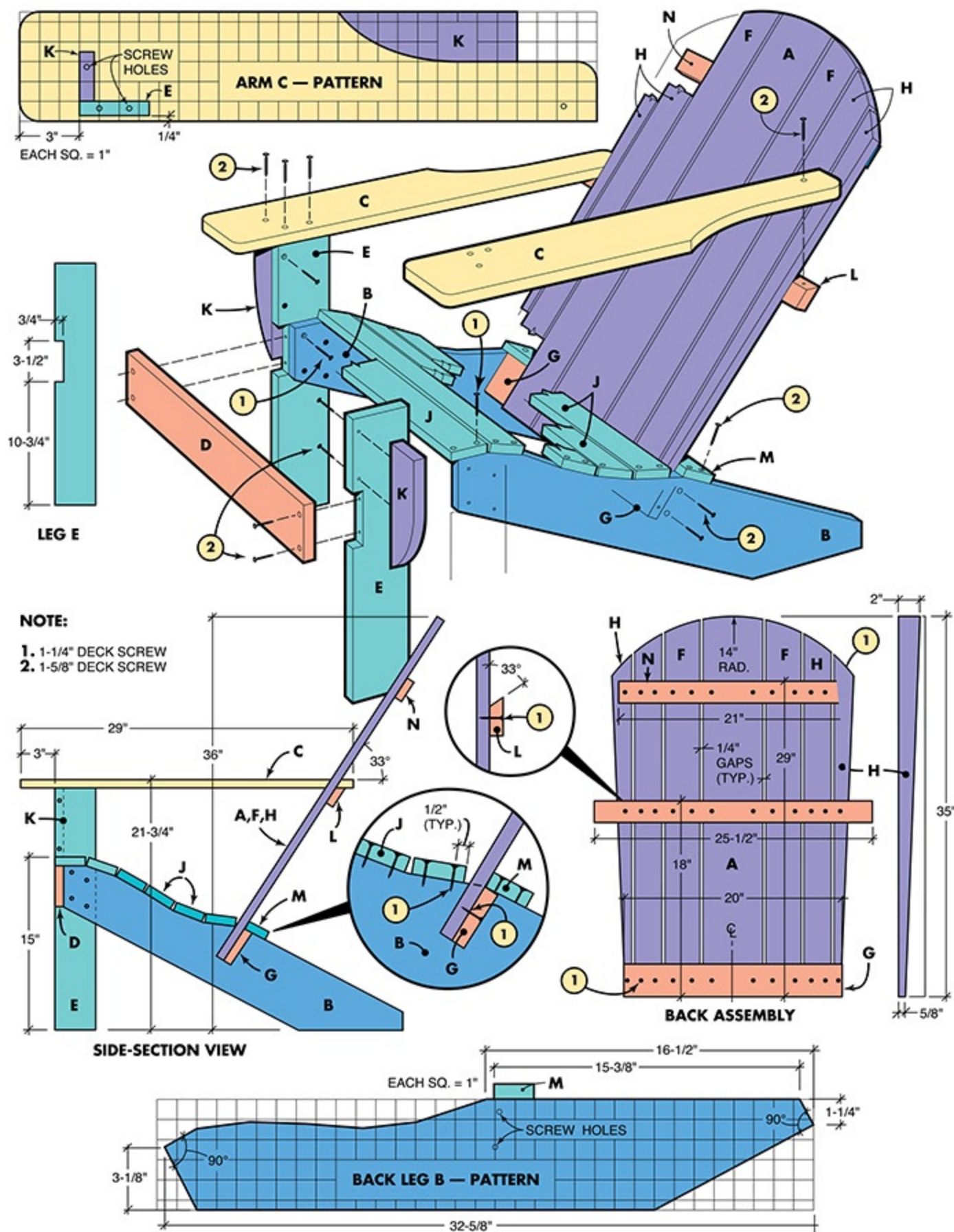
FIG. A ADIRONDACK CHAIR
